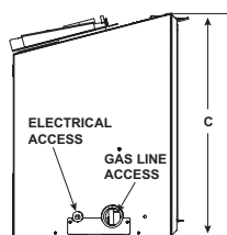
Left View
