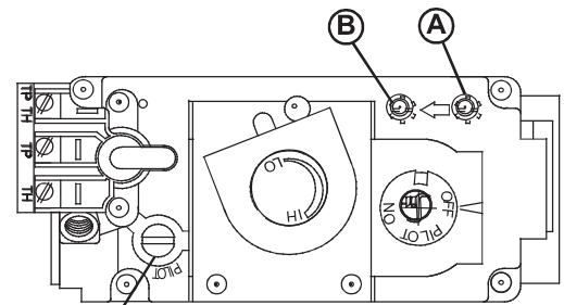
PILOT SCREW
