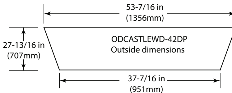
Figure 3. Drain pan dimensions
