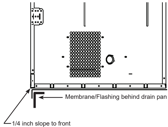
Figure 2. Drain pan installed under appliance.
