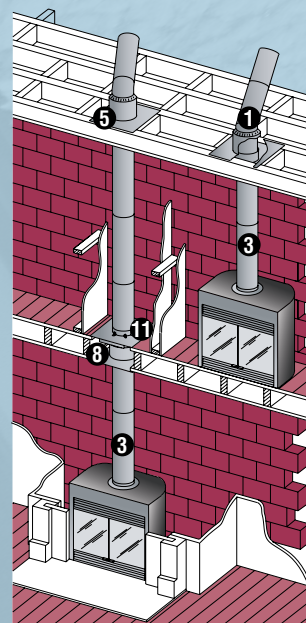
Chimney with several fireplaces
